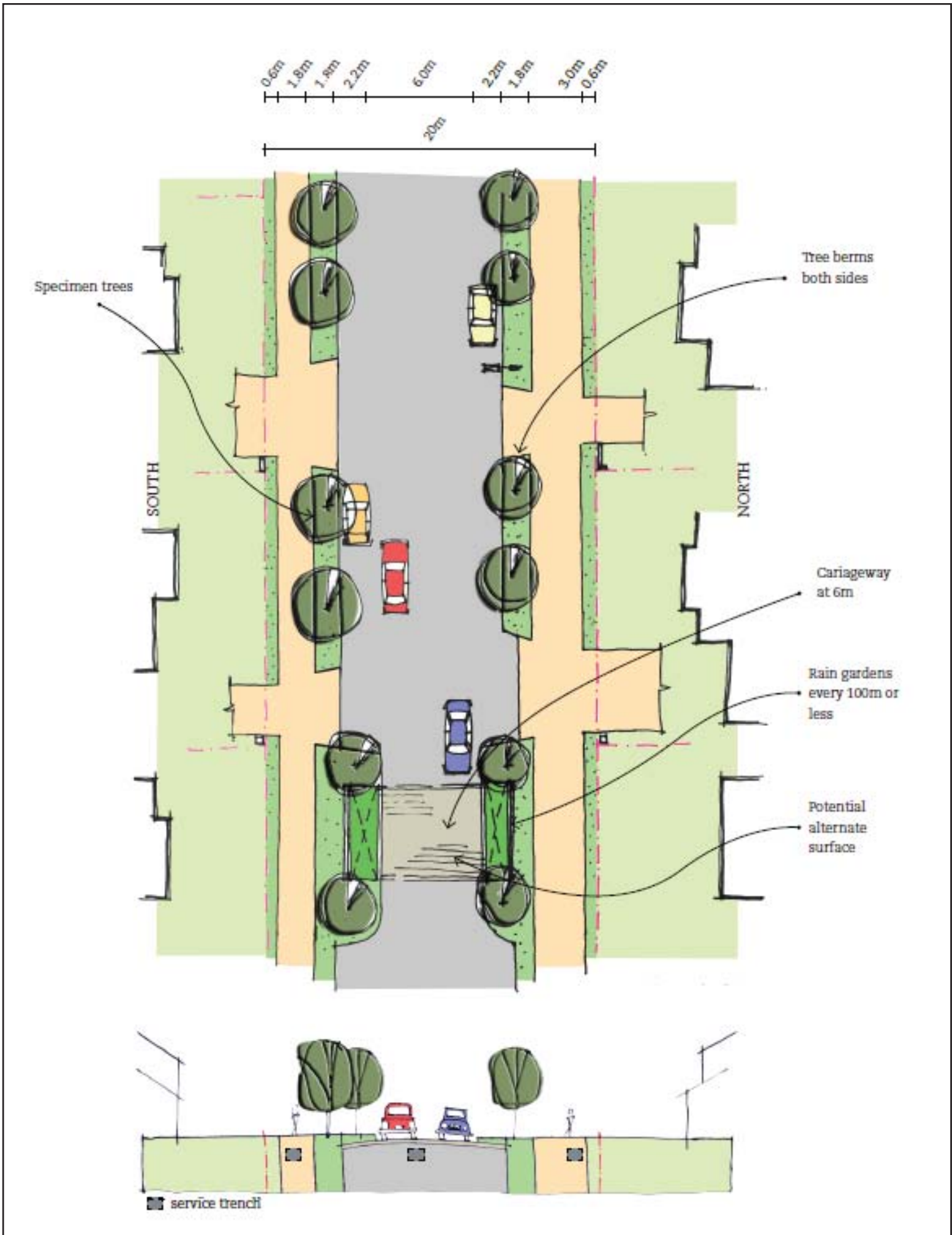
Figure 5- Road Typology B - Ihumatao Quarry Road
